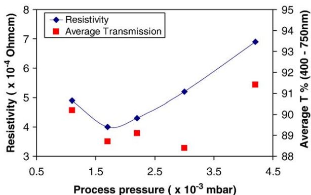
Fig. 5. The effect of process pressure on the optical and electrical properties of ITO.
