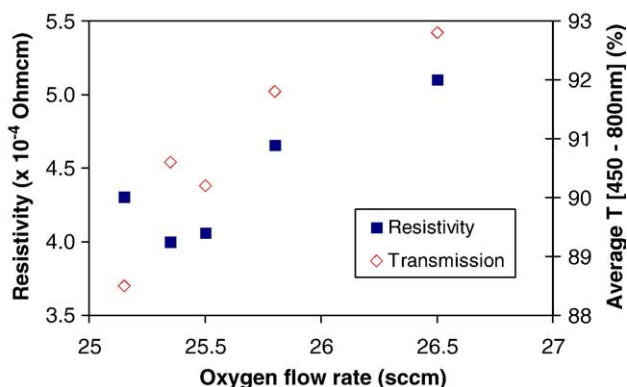
Fig. 2. The dependence of resistivity and transmission on oxygen flow rate.
