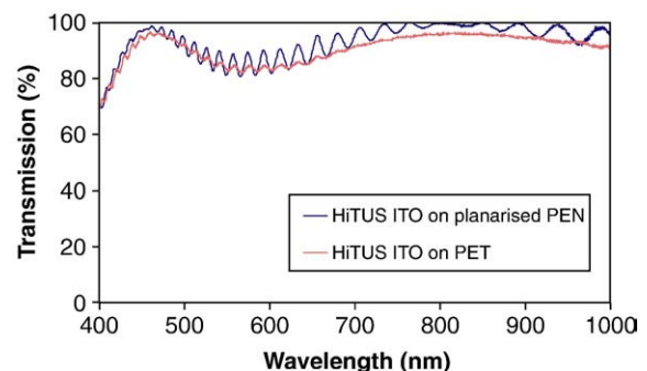
Fig. 4. Transmission profiles of ITO deposited onto PET and planarised PEN flexible substrates. The high frequency ripples are due to an adhesion layer that the manufacturers put in the reverse side of the substrate.
