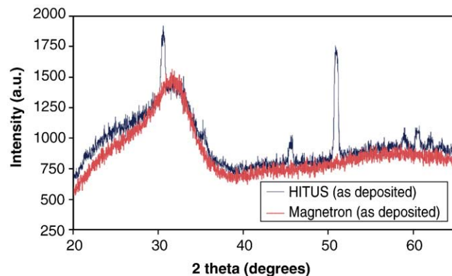
Fig. 7. XRD results indicating that ITO films deposited using HiTUS show some crystallographic structure even at low substrate temperatures. A similar ITO film deposited using magnetron sputtering is included for comparison.
