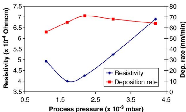
Fig. 6. The effect of process pressure on the resistivity and deposition rate of ITO.
