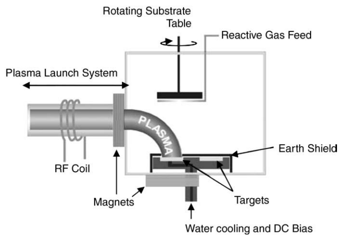
Fig. 1. Schematic showing the HiTUS system. Electromagnets at the exit of the PLS enhance and steer the plasma onto the target.
