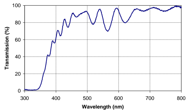
Figure 6. Transmission profile of a complete EL device with ITO-Y 2 O 3 -ZnS:Mn-Y 2 O 3 -ITO structure.
