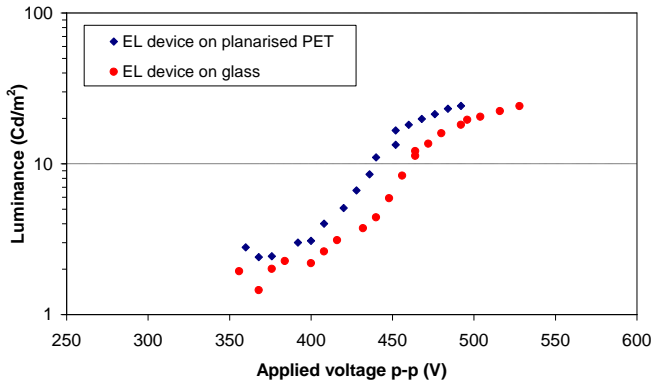
Figure 7. EL intensity as a function of applied voltage for a device deposited onto planarised PET at room temperature with no post deposition annealing.
