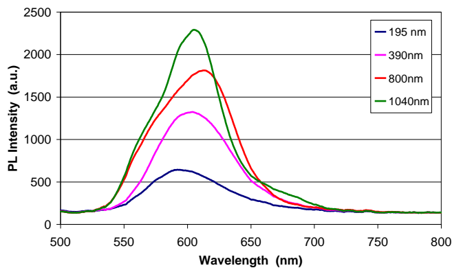
Figure 5. Improvement of PL intensity with increased film thickness
