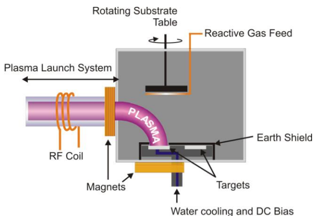
Figure 1. A schematic showing the HiTUS system
