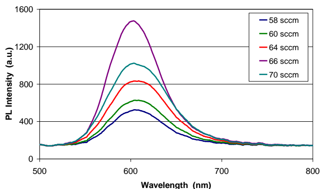
Figure 2. Variation of PL with H 2 S gas flow.
