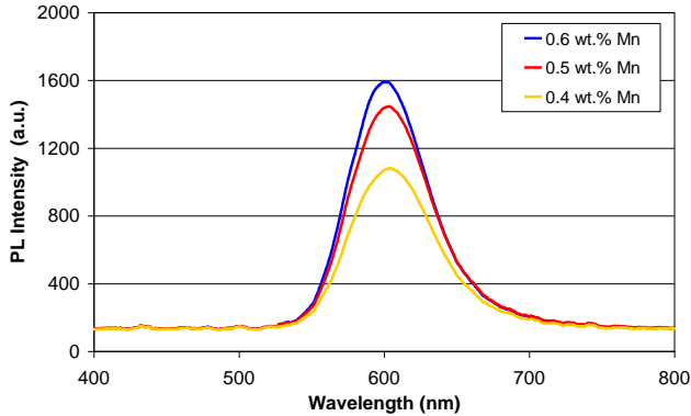
Figure 4. The effect of varying concentrations of Mn in the Zn target
