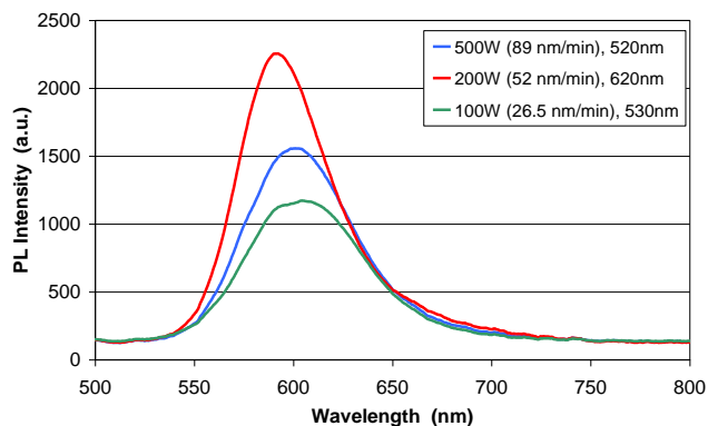
Figure 3. Variation of PL with target power
